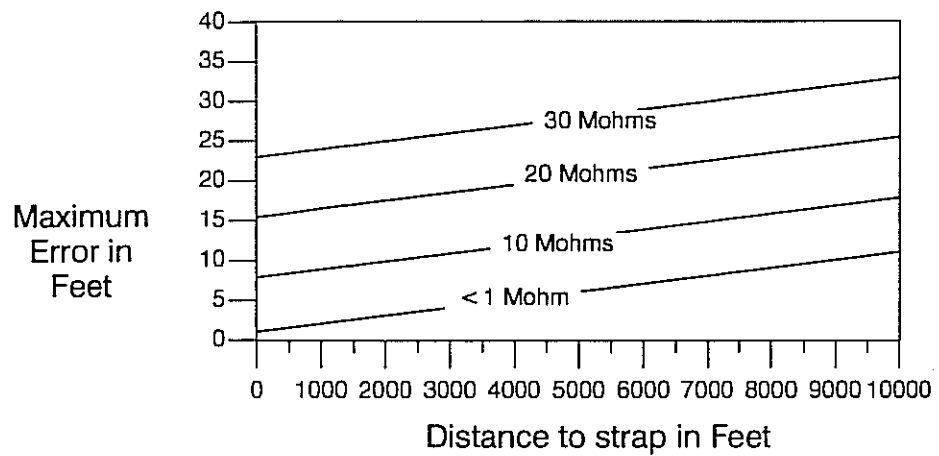
Accuracy for 24 Gauge for Various Fault Resistances
