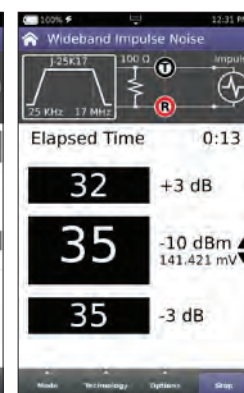
Wideband Impulse Noise
