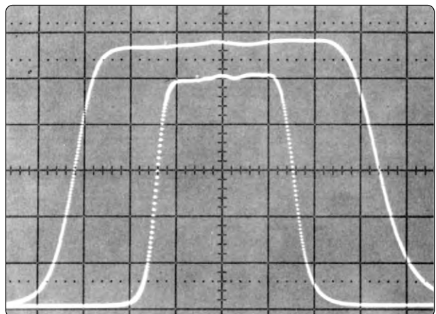
Swept response of a bandpass filter using span sweep.
