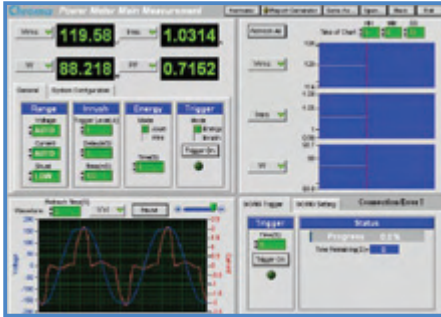
66200 Softpanel
