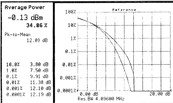
Complementary cumulative-distribution function curves
