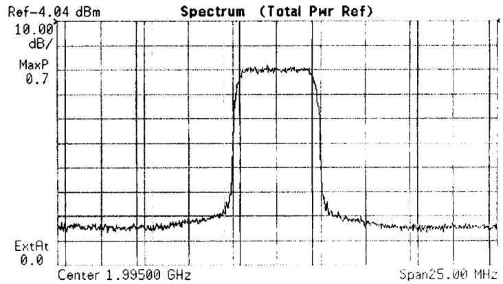
W-CDMA adjacent channel power ratio (ACPR) measurement
