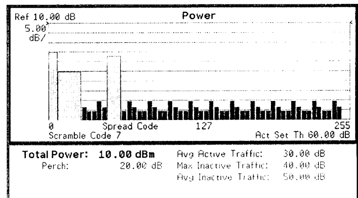
Code domain power measurement
