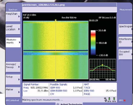
Interference analyzer
