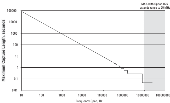
Figure 3. MXA and EXA capture length
