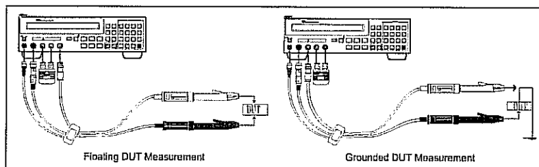
Floating and grounded DUT measurement
