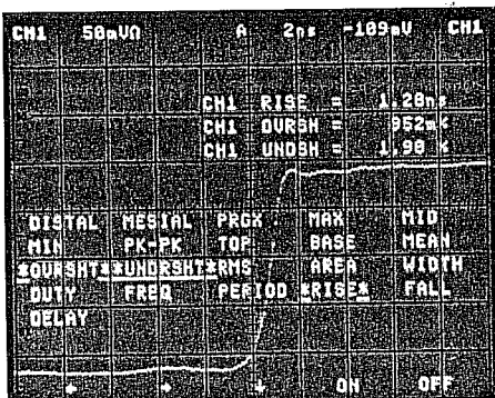
The auto measure feature provides a menu of the 21 measurements that you can select. Here the user selected rise time, undershoot, and overshoot measurements of the waveform on channel 1.
